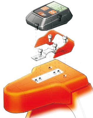
Schematic exploded view of product configuration
